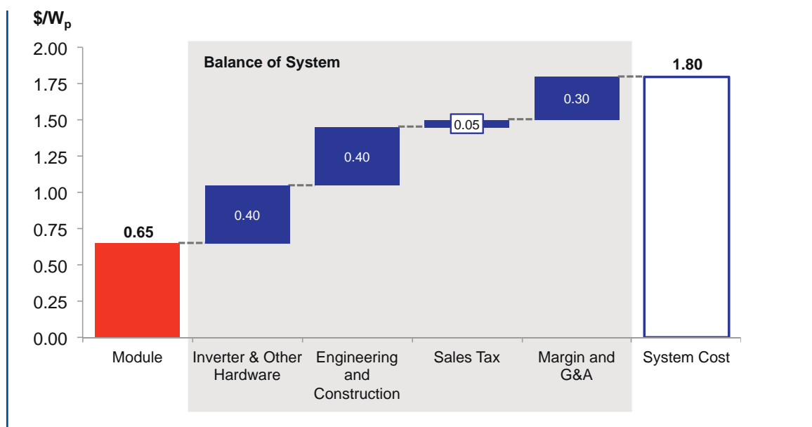
Figure 4.7 Stair Step Build-Up of Estimated Costs for a Utility-Scale PV System iii
