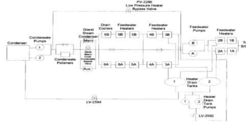
Figure 1 Simplified Condensate and Feedwater System IS 1292 SER 10-96
